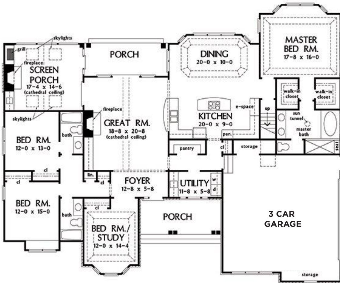
FLOOR PLAN
